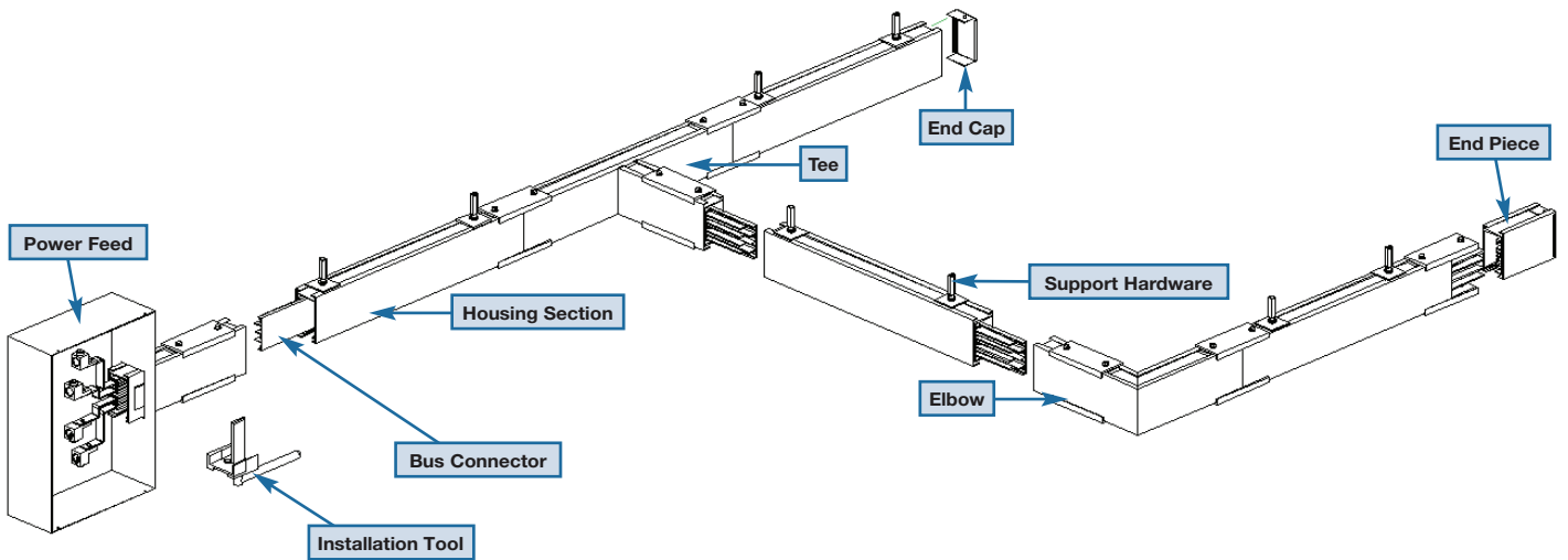
Fig: GM225Amp ceiling mounted system, also available for raised floor plenum design
